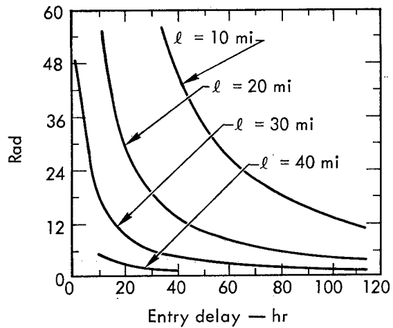
Fig. A-8. Total radiation exposure after area-entry delay, for various distances from ground zero of a 100-kt detonation. The expected march rate is 1 mph.
